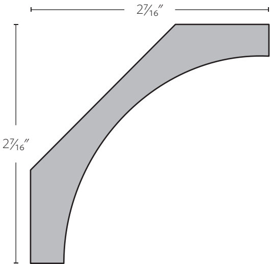
SWD 502 | 7/8" x 3 1/2" | 45/45
