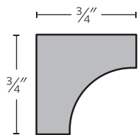
SWD 500 | 3/4" x 3/4"
