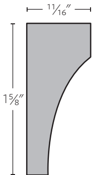
SWD 501 | 1 1/16" x 1 5/8"
