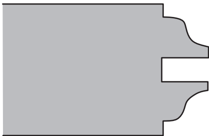
SWD 364 | 1 3/8"
