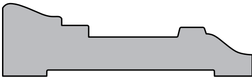
SWD 1042 | \frac{3}{4}" \times 2\frac{9}{16}"
