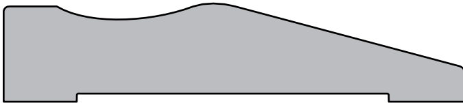
SWD 047 | \frac{3}{4}'' \times 3\frac{1}{2}''
