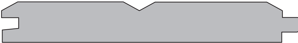
SWD 615 | \frac{3}{4} " x 5\frac{7}{16} " | 5\frac{1}{8} " Lay
