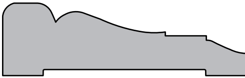
SWD 1035 | 3/4" x 2 1/2"
