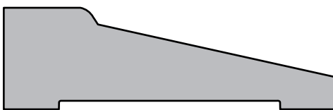
SWD 1038 | 3/4" x 2 7/16"
