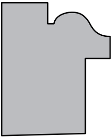
SWD 492 1 1/8" x 1 3/8"
