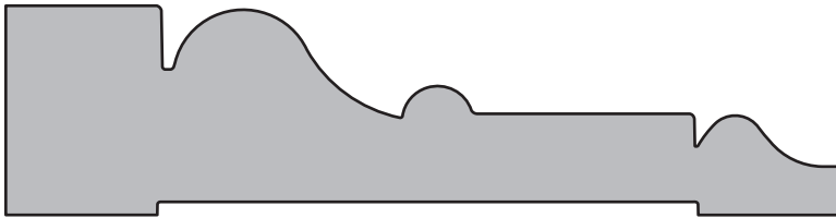
SWD 1125 | 1" x 4"
