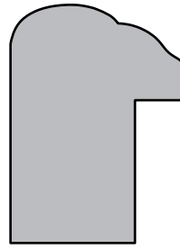
SWD 493 1" x 1 3/8"
