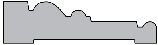
SWD 1061 | 3/4" x 2 3 / 4 "
