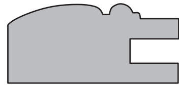
SWD 847 | 2\frac{5}{32} " x 1\frac{3}{4} "
