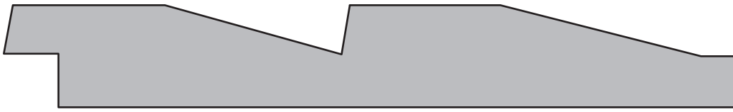
SWD 813 | \frac{3}{4}'' \times 5\frac{3}{8}'' | Siding
