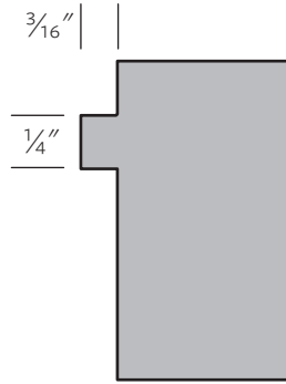
SWD 806-B | 1" x 1 1/2"
