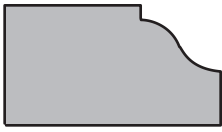
SWD 700-S | \frac{5}{8} " x 1\frac{1}{8} " | Shelf Edge
