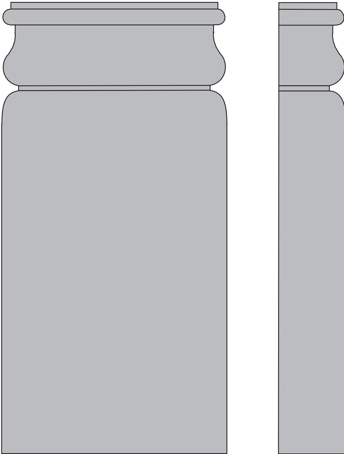
SWD 665 | 1\frac{1}{8}'' \times 3\frac{3}{4}'' \times 7\frac{1}{2}'' Also Available | 1\frac{1}{8}'' \times 6\frac{1}{8}'' \times 7\frac{1}{2}''
