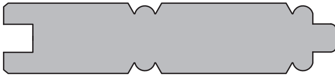
SWD 620 | \frac{3}{4}'' x 3\frac{1}{2}'' | 3\frac{1}{4}'' Lay
