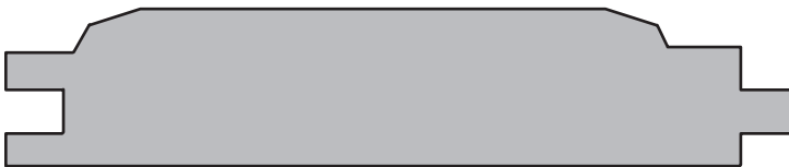
SWD 603 | \frac{3}{4} " x 3\frac{3}{4} " | 3\frac{1}{2} " Lay
