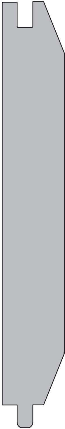
SWD 618 1 \frac{1}{16} " x 7 \frac{1}{4} " 6 \frac{13}{16} " Lay
