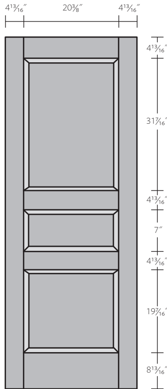
Three Panel Door
