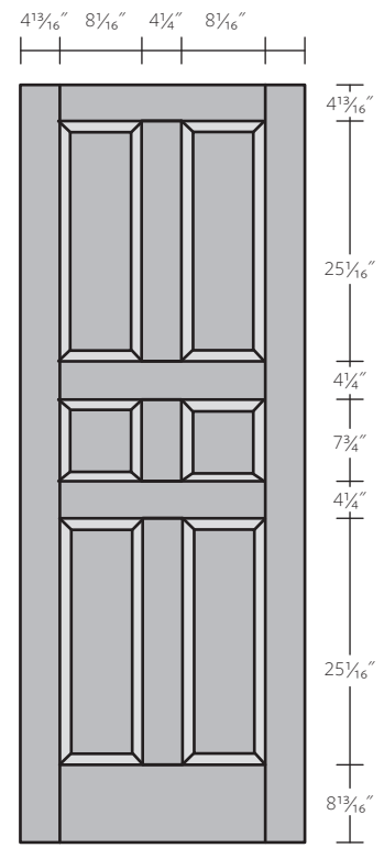
Six Panel Door (Alternate)
