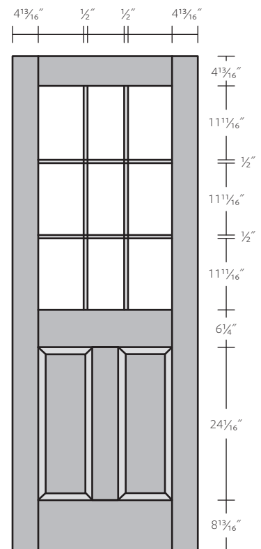
Two Panel Nine Light Glass Door
