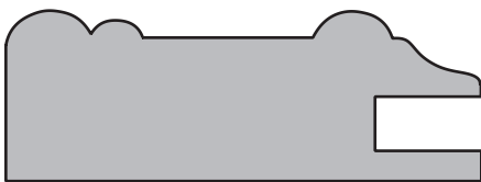
SWD 850 | 25\frac{5}{32}" \times 2\frac{1}{4}"
