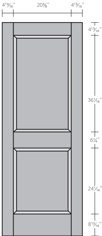
Two Panel Door
