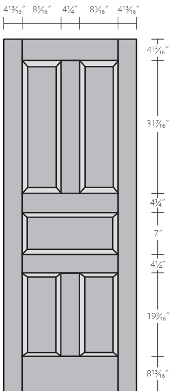
Five Panel Door
