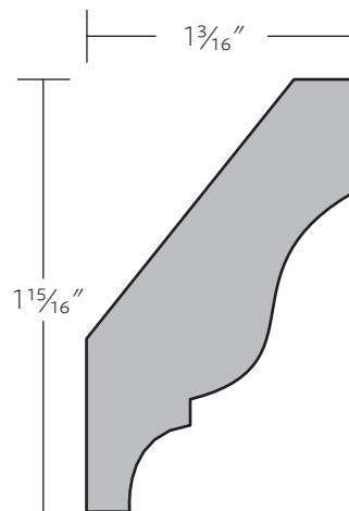
SWD 540 | \frac{3}{4}" \times 2\frac{1}{4}" | 38/52
