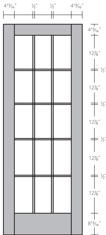
Fifteen Light Glass Door
