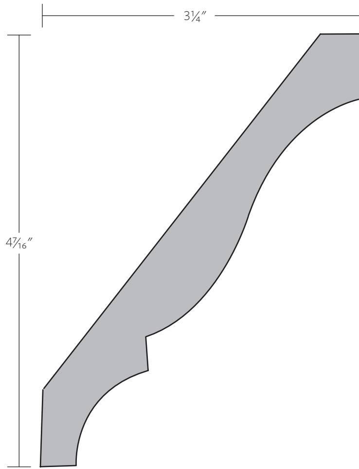
SWD 530 | \frac{3}{4}" \times 5\frac{1}{2}" | 38/52
