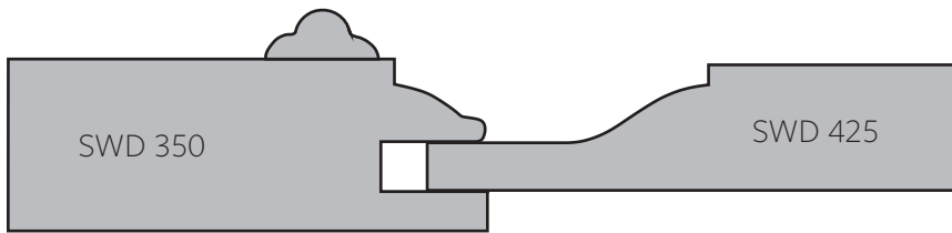
SWD 3168 | Applied Moulding
