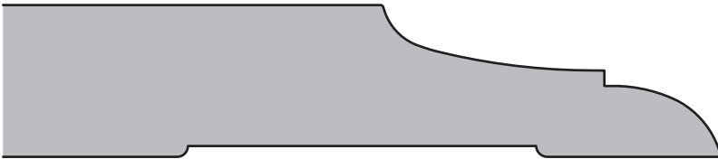
SWD 2133 | \frac{7}{8} " x Customer Specs
