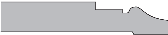
SWD 2051 | 1\frac{1}{16} " x Customer Specs
