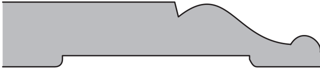
SWD 227 | 1\frac{1}{16} " x Customer Specs
