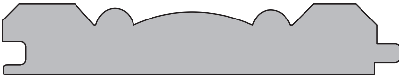
SWD 602 | \frac{3}{4} " x 4\frac{1}{4} " | 4" Lay
