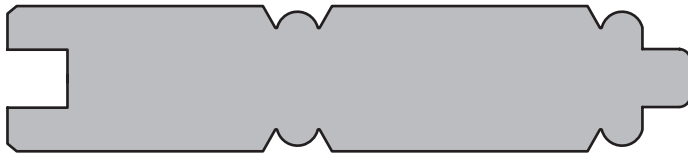
SWD 620 | \frac{3}{4}'' \times 3\frac{1}{2}'' | 3\frac{1}{4}'' Lay
