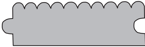
SWD 619 | \frac{3}{4}'' \times 2\frac{1}{2}'' | 2\frac{1}{4}'' Lay
