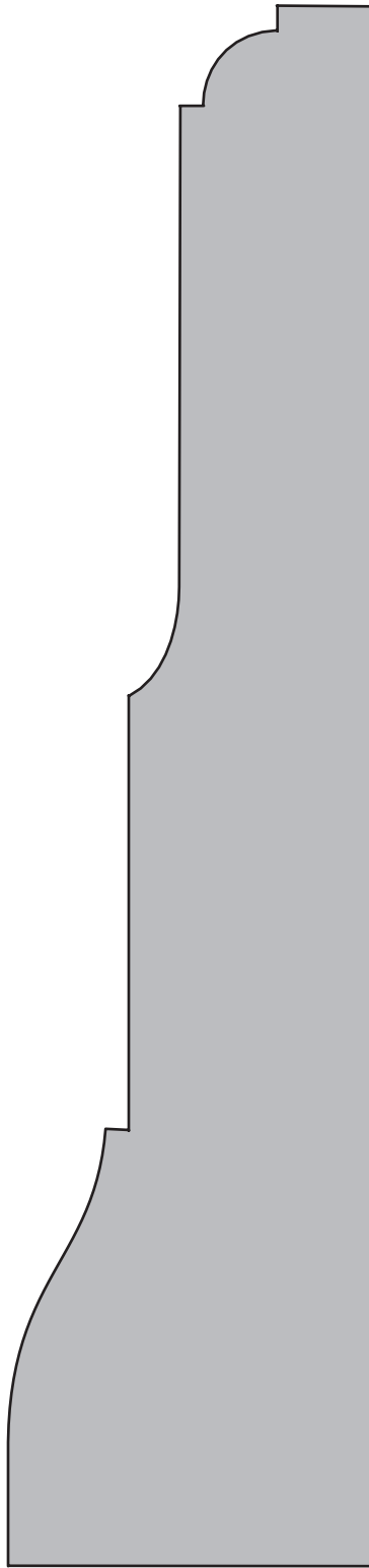
SWD 664 | 1 7/8" x 8"
