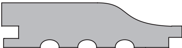
SWD 610 | \frac{3}{4} " x 3" | 2\frac{3}{4} " Lay
