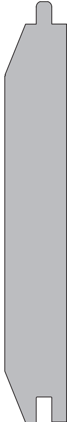
SWD 618 | 1\frac{1}{16}'' \times 7\frac{1}{4}'' | 6\frac{3}{16}'' Lay
