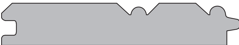
SWD 604 | \frac{3}{4} " x 4\frac{1}{4} " | 4" Lay
