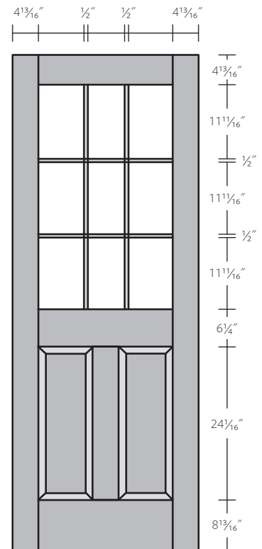
Two Panel Nine Light Glass Door
